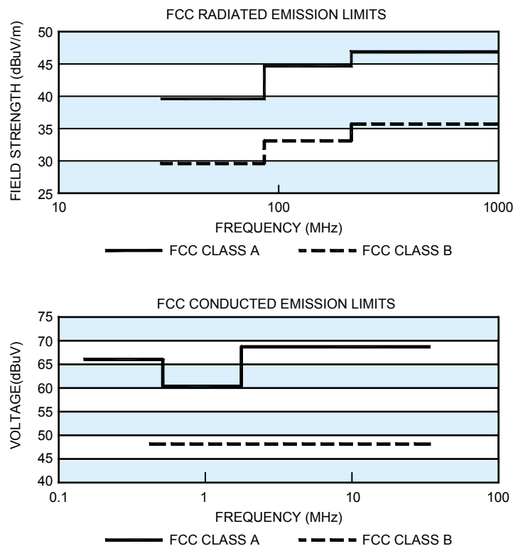
Chart 1.0 FCC Standards for maximum allowable radiated emissions
