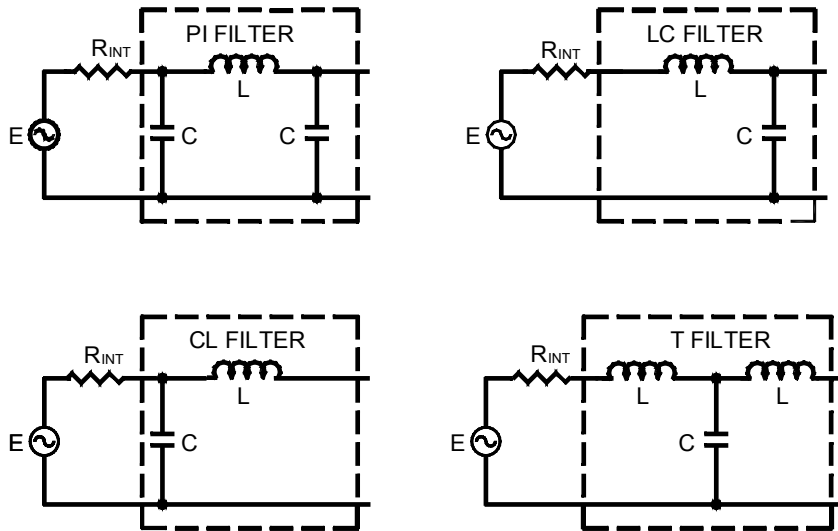
Fig. 3.0 Different circuit configurations
