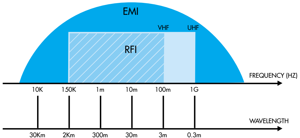
Fig. 1.0 Frequency range for EMI and RFI
