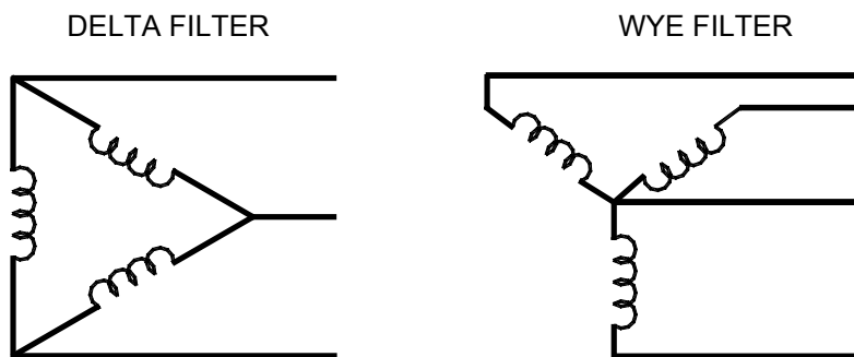
Fig. 4.0 Three Phase configurations.
