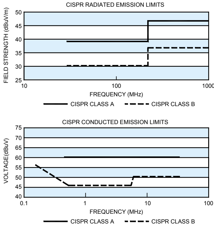
Chart 2.0 CISPR Standards for maximum allowable emissions
