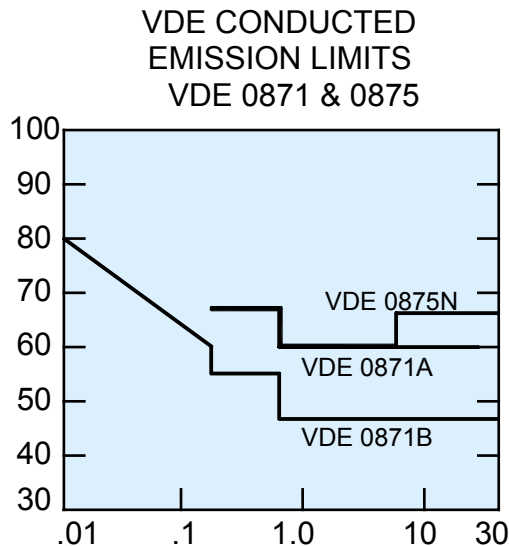
Chart 3.0 VDE Standards for maximum allowable emissions
